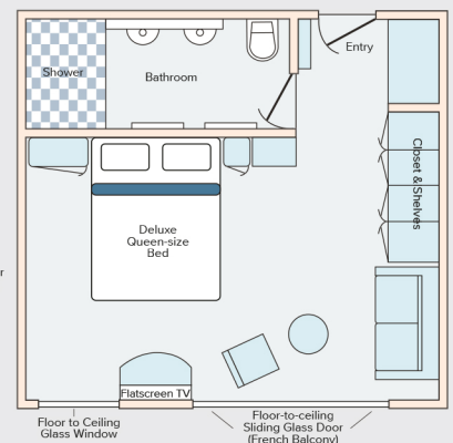
Floor plan of an Owner's Suite Category: OS 258 square feet/24 square metres
