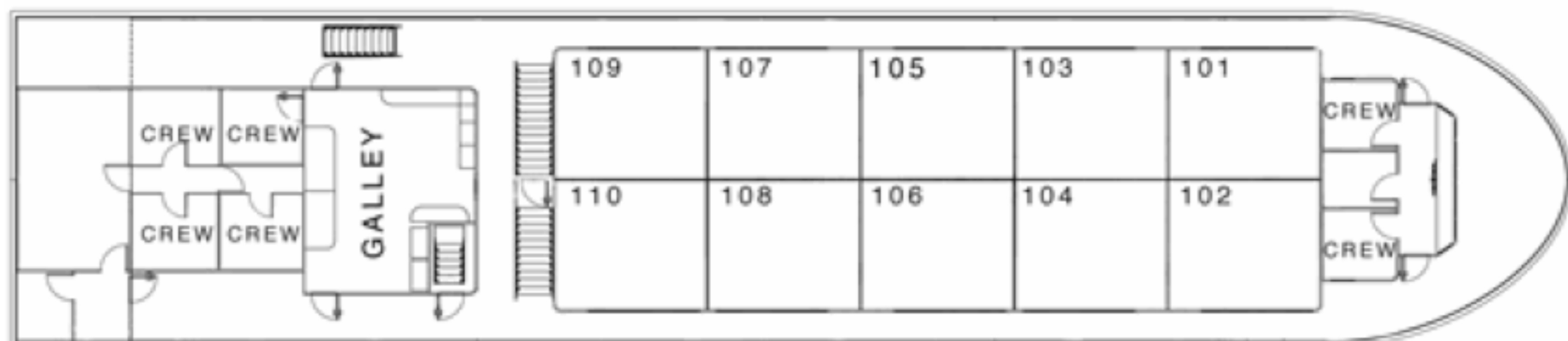
MAIN DECK
